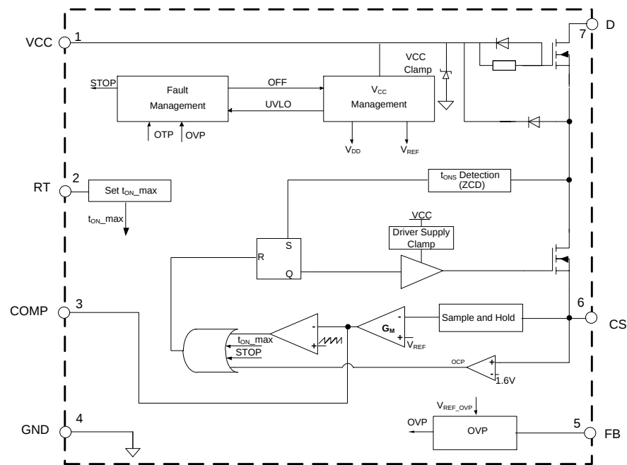
AL1692-20C with MOSFET
